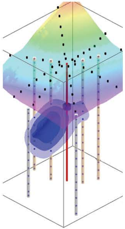
The image above was produced from data acquired during a pressurized injection monitoring project. The data were inverse modeled to produce volumetric images of solution coverage. This image shows the progression of fluid movement at three different times during the injection at a depth of 110 feet (note 3 blue color changes in plume injection).
