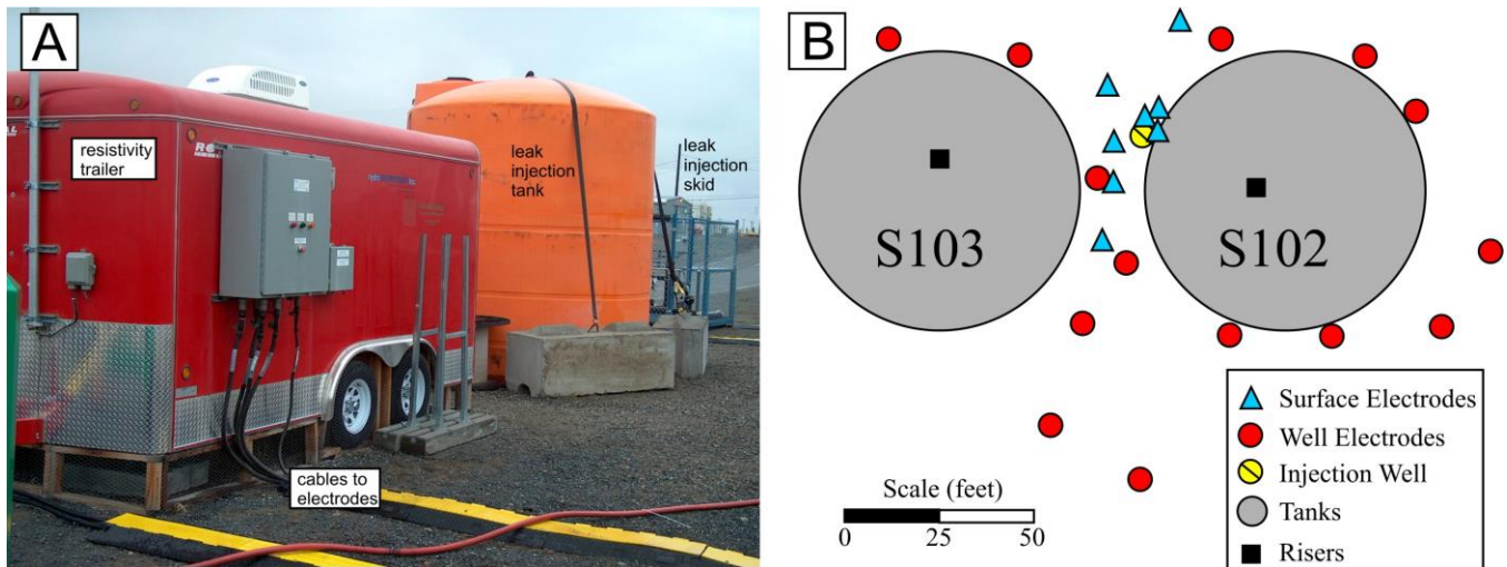
Figure 6: A) Environmentally controlled trailer housing the HRR-LDM data acquisition equipment and electronics. Photo taken during the leak injection test at S-102. B) Layout of the HRR-LDM electrodes around tank S-102 and the injection well.
